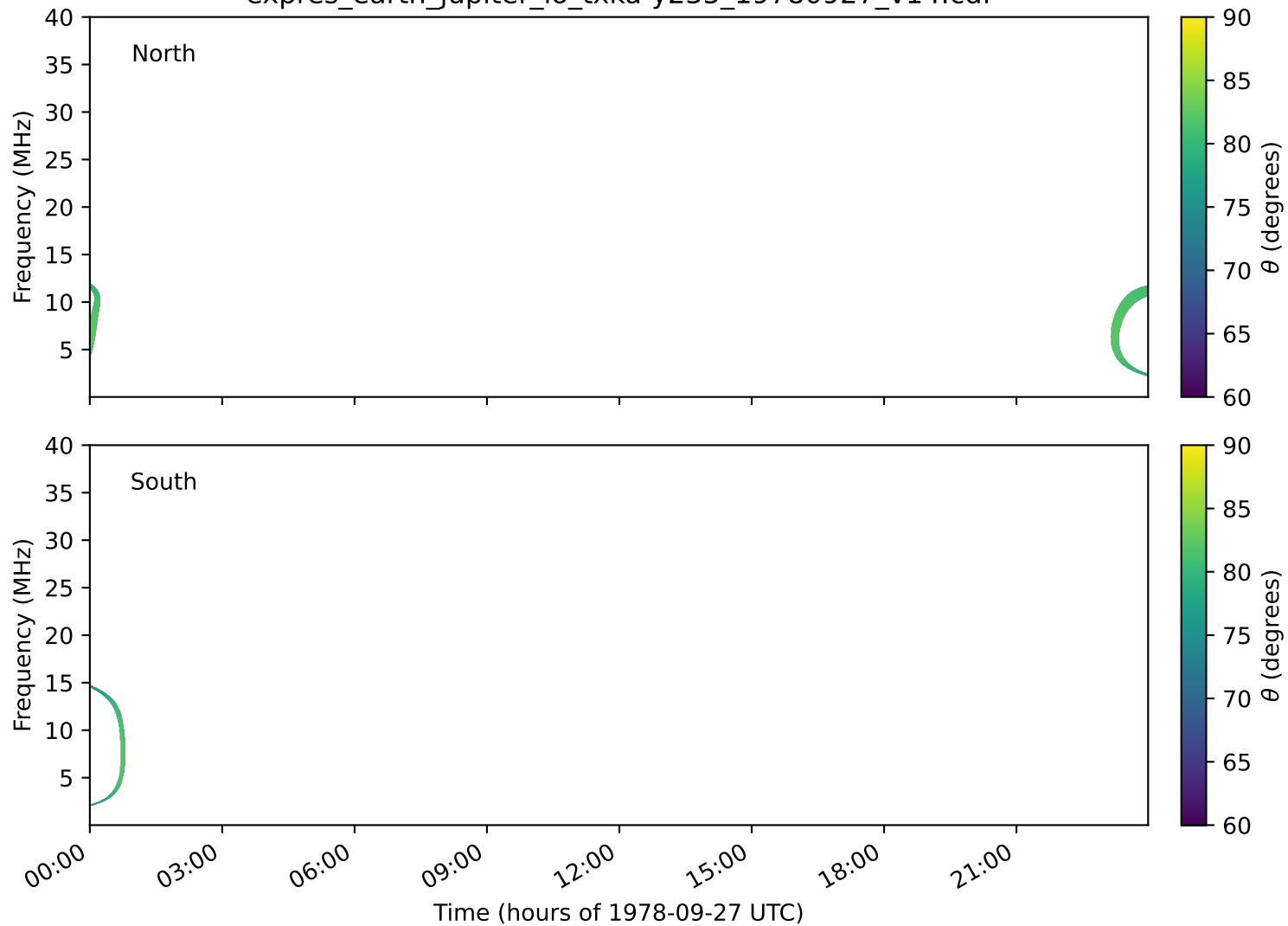
expres_earth_jupiter_io_txka-y235_19780927_v14.cdf
