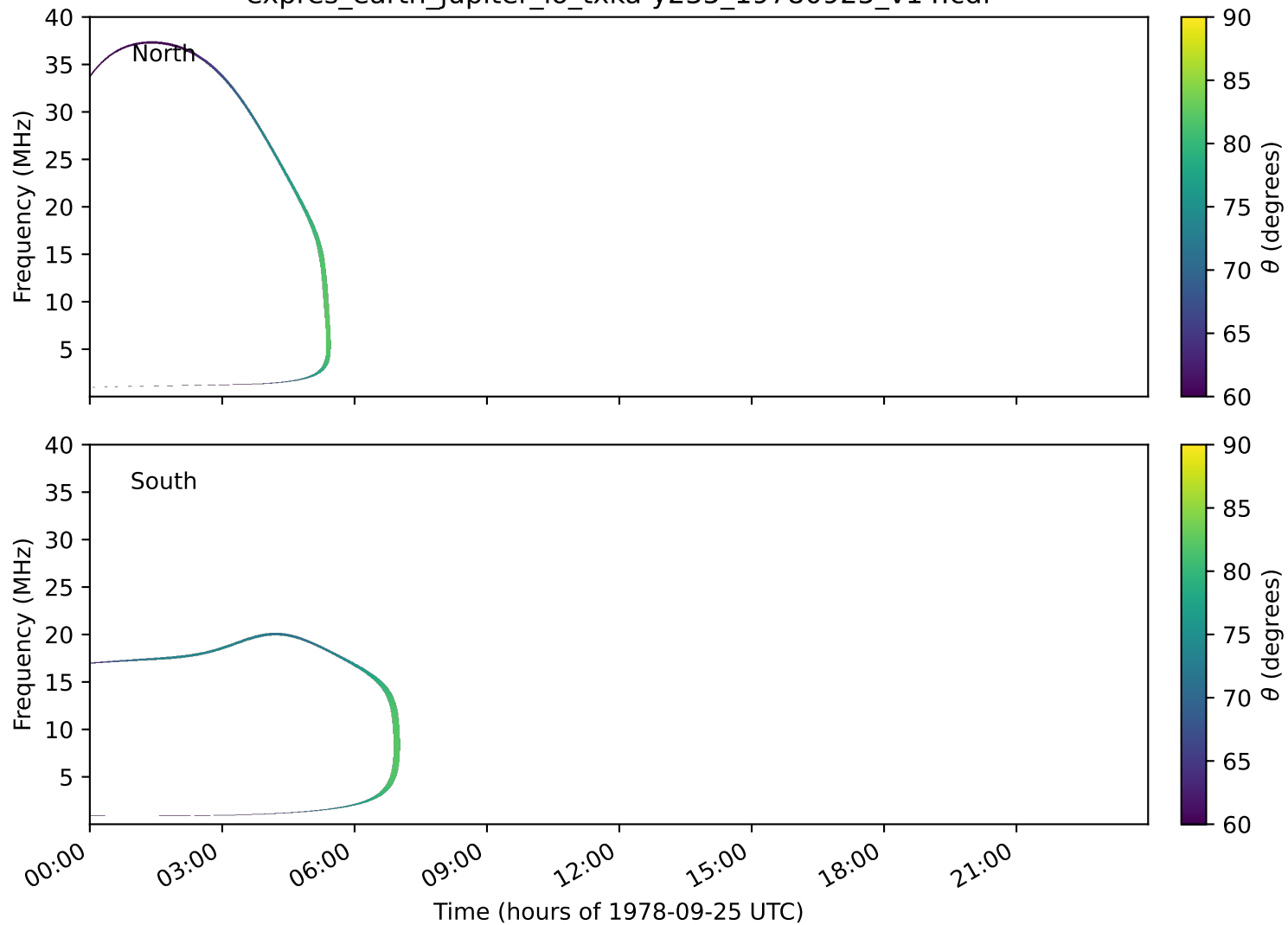
expres_earth_jupiter_io_txka-y235_19780925_v14.cdf
