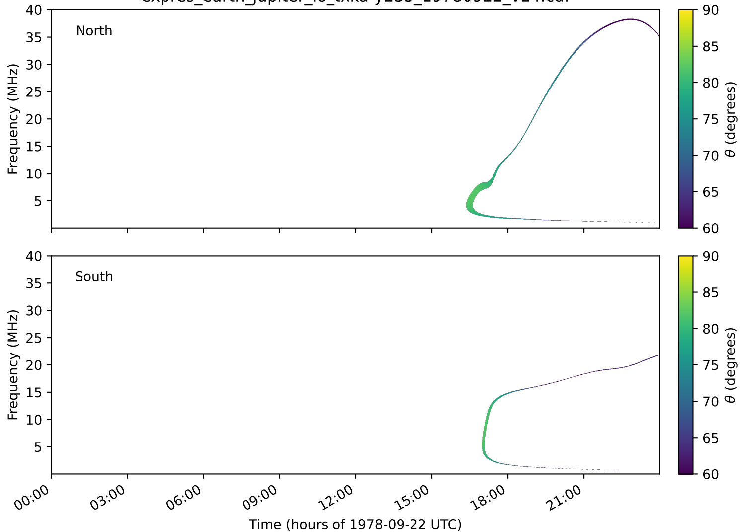
expres_earth_jupiter_io_txka-y235_19780922_v14.cdf
