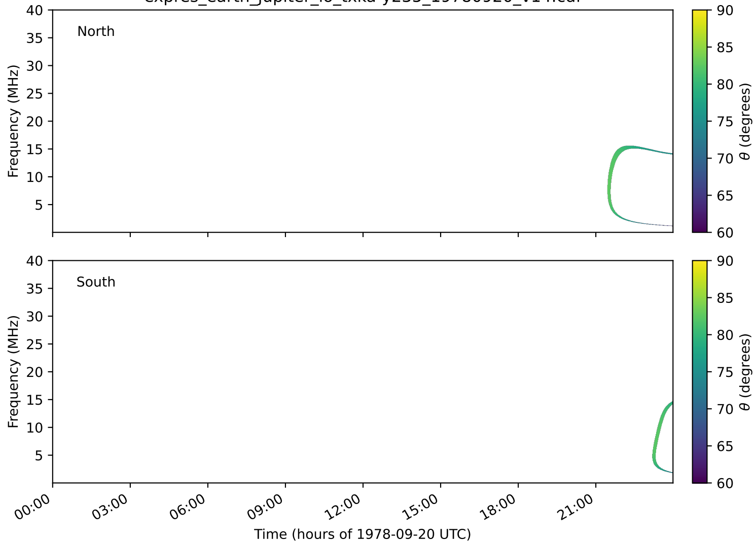
expres_earth_jupiter_io_txka-y235_19780920_v14.cdf
