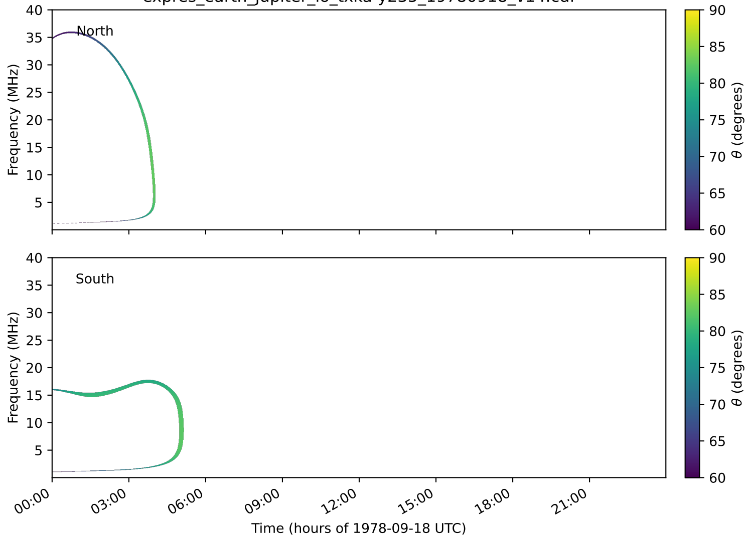
expres_earth_jupiter_io_txka-y235_19780918_v14.cdf
