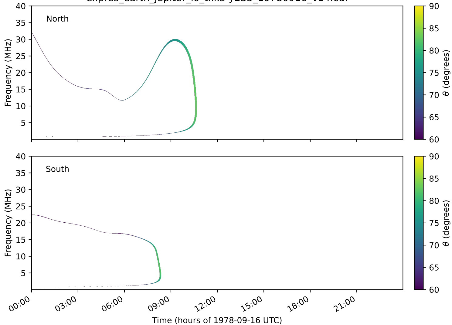
expres_earth_jupiter_io_txka-y235_19780916_v14.cdf
