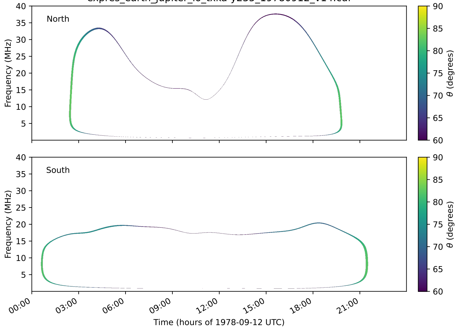
expres_earth_jupiter_io_txka-y235_19780912_v14.cdf
