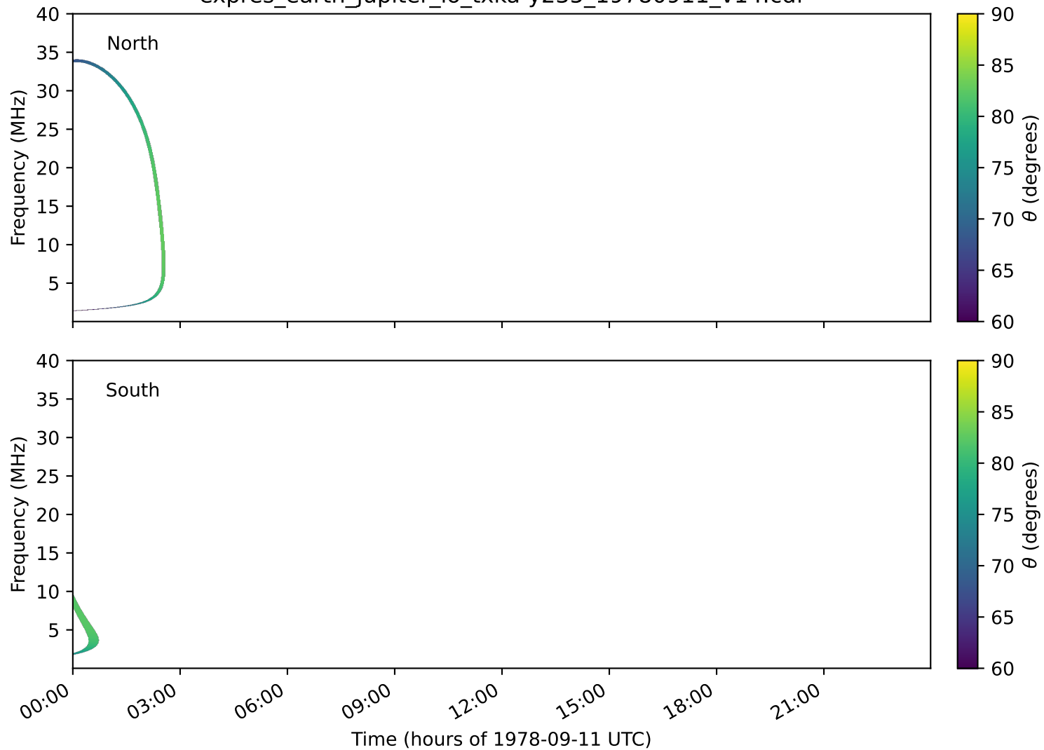
expres_earth_jupiter_io_txka-y235_19780911_v14.cdf
