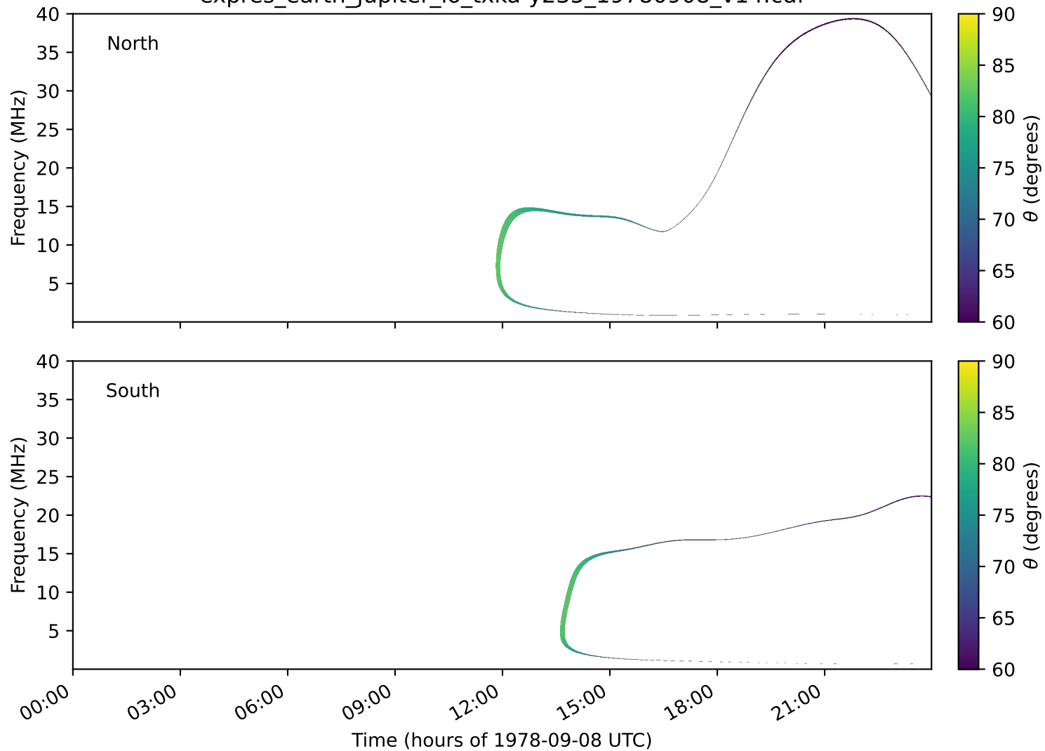
expres_earth_jupiter_io_txka-y235_19780908_v14.cdf
