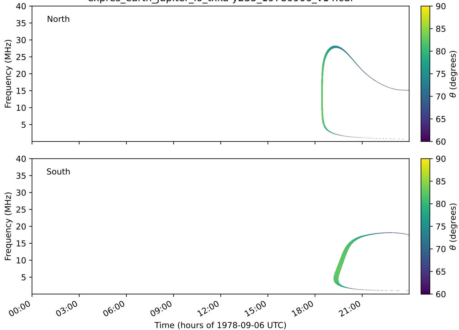
expres_earth_jupiter_io_txka-y235_19780906_v14.cdf
