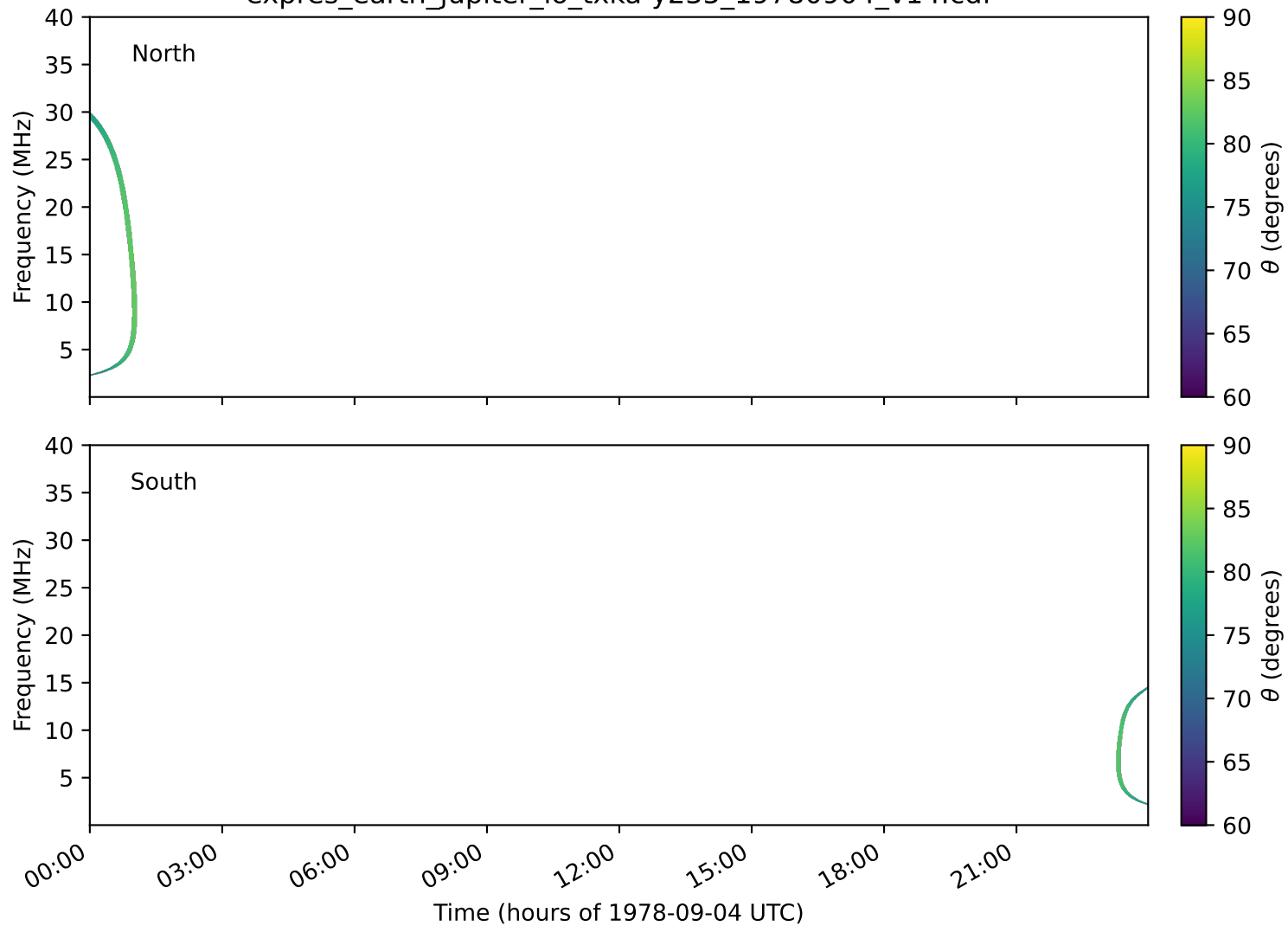
expres_earth_jupiter_io_txka-y235_19780904_v14.cdf
