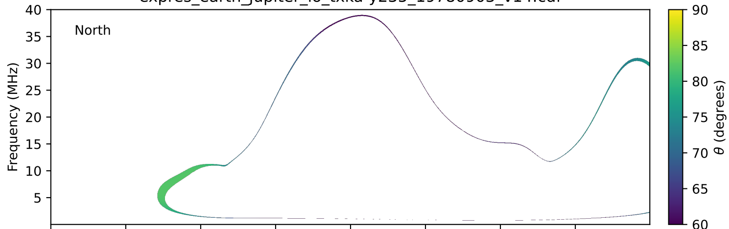
expres_earth_jupiter_io_txka-y235_19780903_v14.cdf
