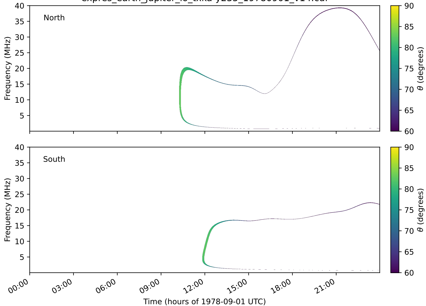
expres_earth_jupiter_io_txka-y235_19780901_v14.cdf
