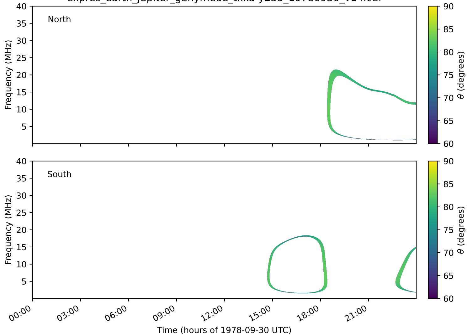
expres_earth_jupiter_ganymede_txka-y235_19780930_v14.cdf
