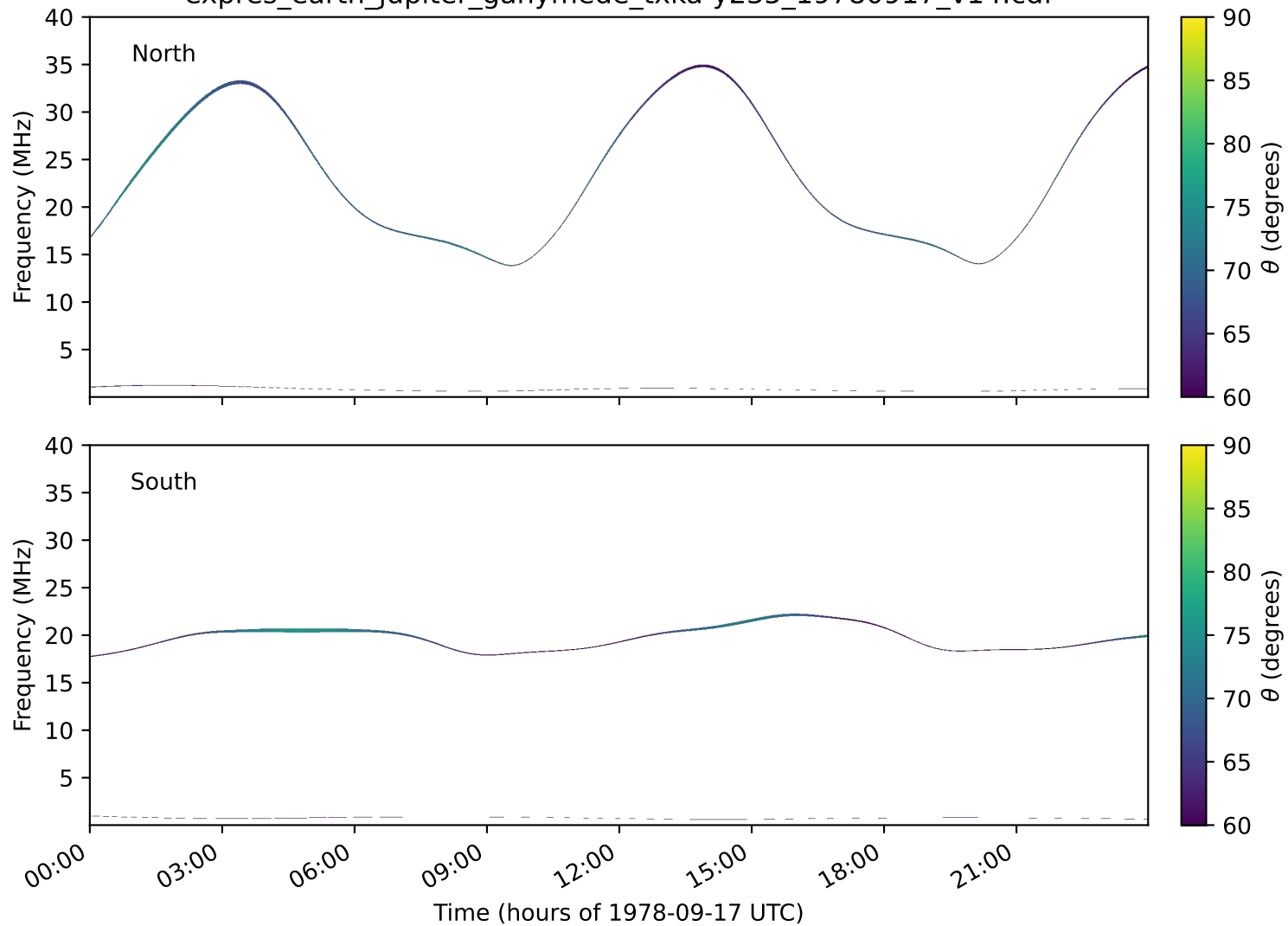
expres_earth_jupiter_ganymede_txka-y235_19780917_v14.cdf
