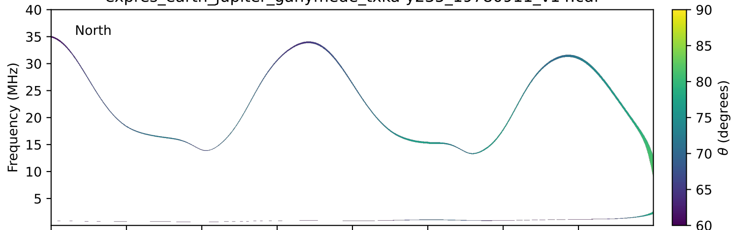
expres_earth_jupiter_ganymede_txka-y235_19780911_v14.cdf
