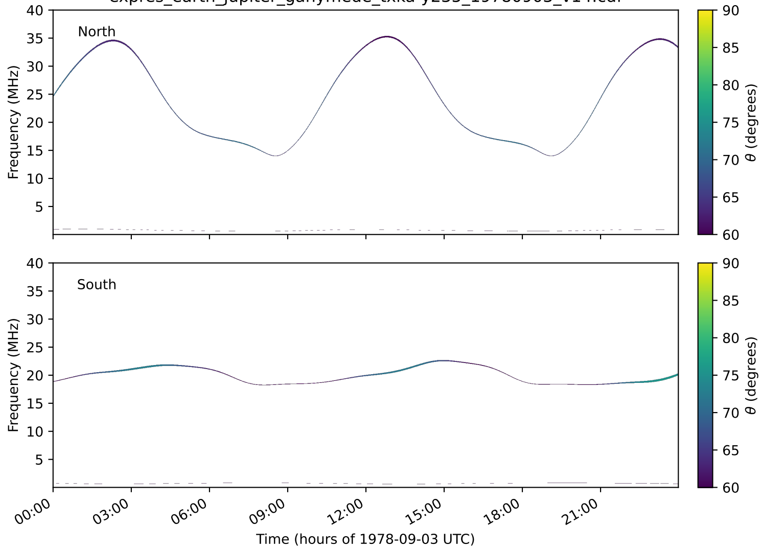
expres_earth_jupiter_ganymede_txka-y235_19780903_v14.cdf
