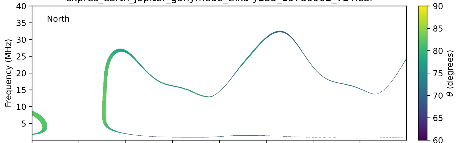
expres_earth_jupiter_ganymede_txka-y235_19780902_v14.cdf
