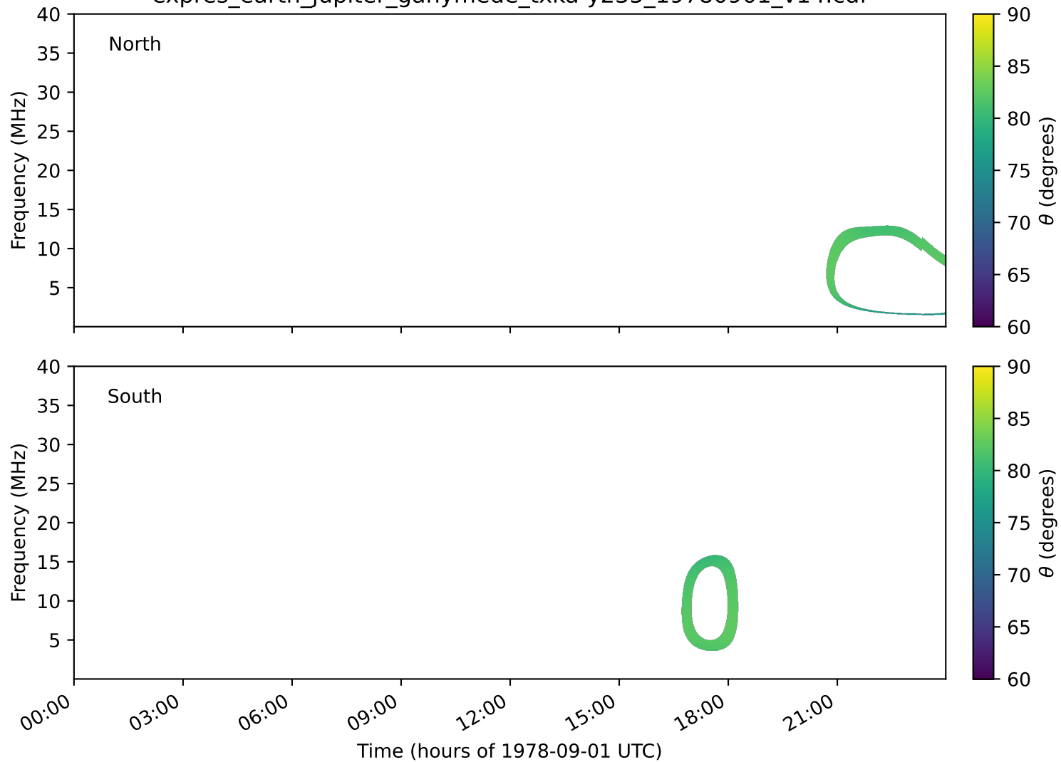
expres_earth_jupiter_ganymede_txka-y235_19780901_v14.cdf
