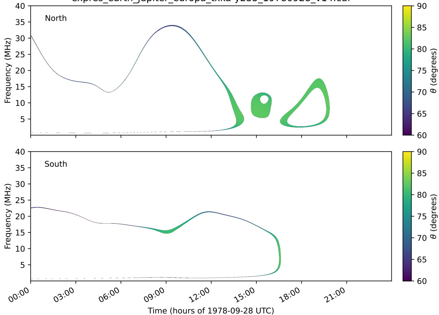
expres_earth_jupiter_europa_txka-y235_19780928_v14.cdf
