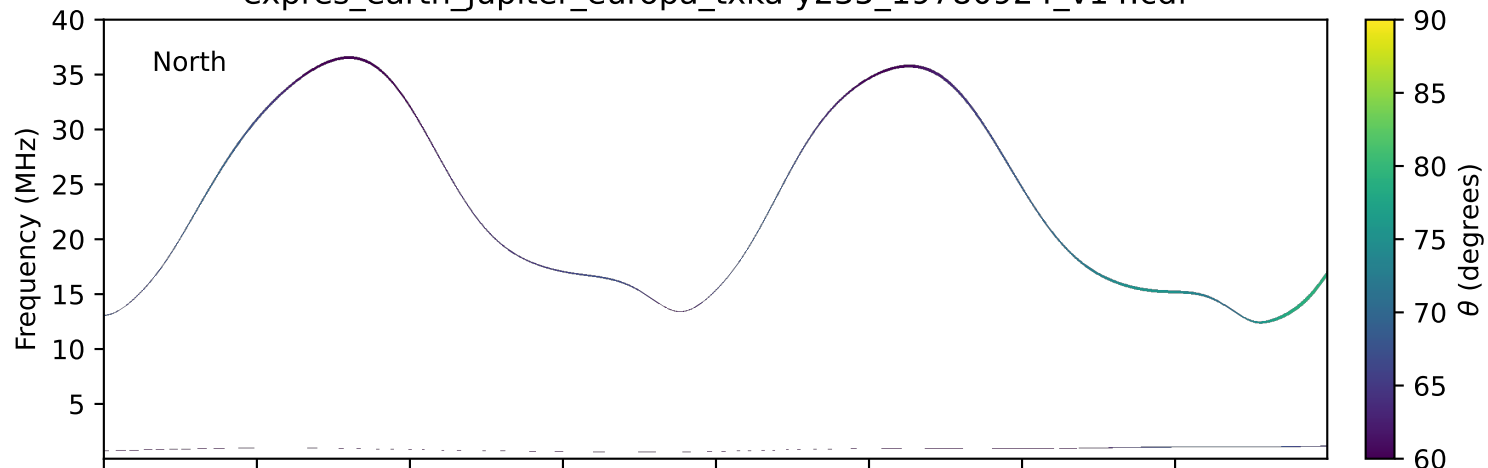
expres_earth_jupiter_europa_txka-y235_19780924_v14.cdf
