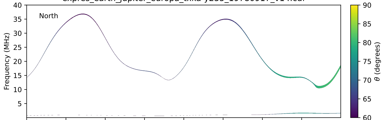
expres_earth_jupiter_europa_txka-y235_19780917_v14.cdf
