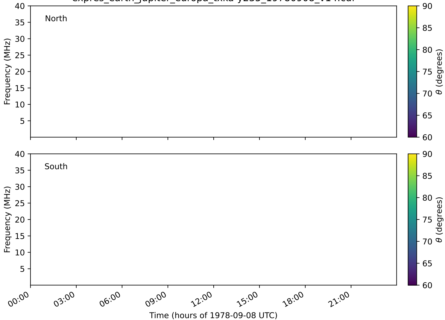
expres_earth_jupiter_europa_txka-y235_19780908_v14.cdf
