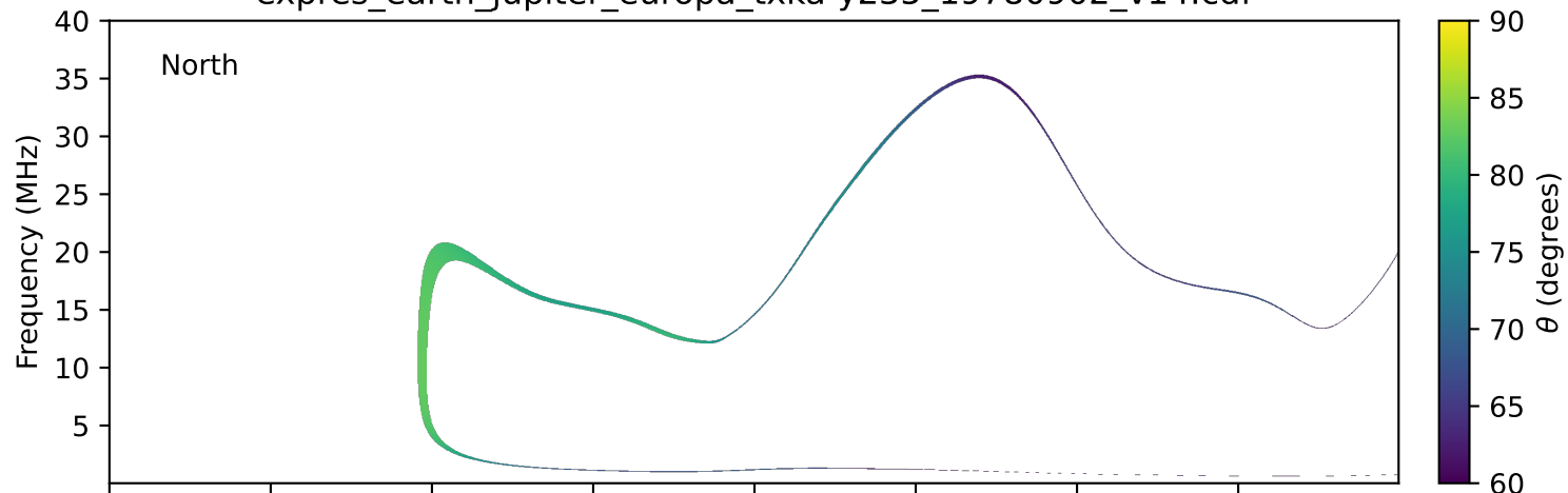
expres_earth_jupiter_europa_txka-y235_19780902_v14.cdf
