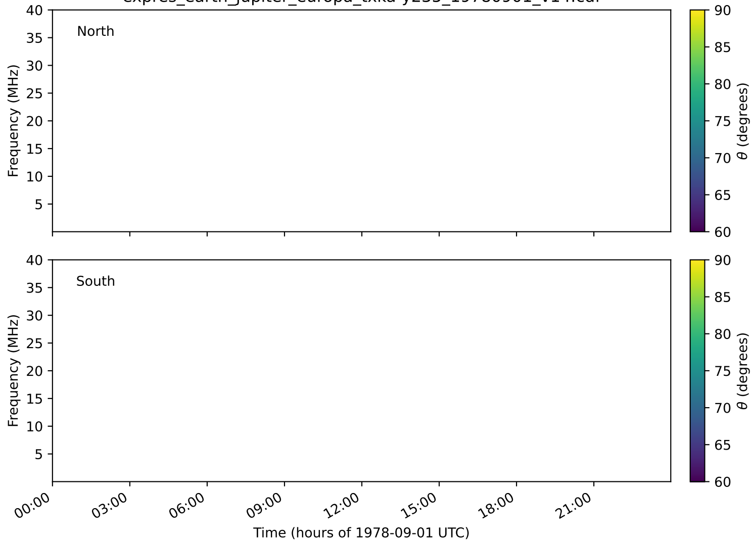
expres_earth_jupiter_europa_txka-y235_19780901_v14.cdf
