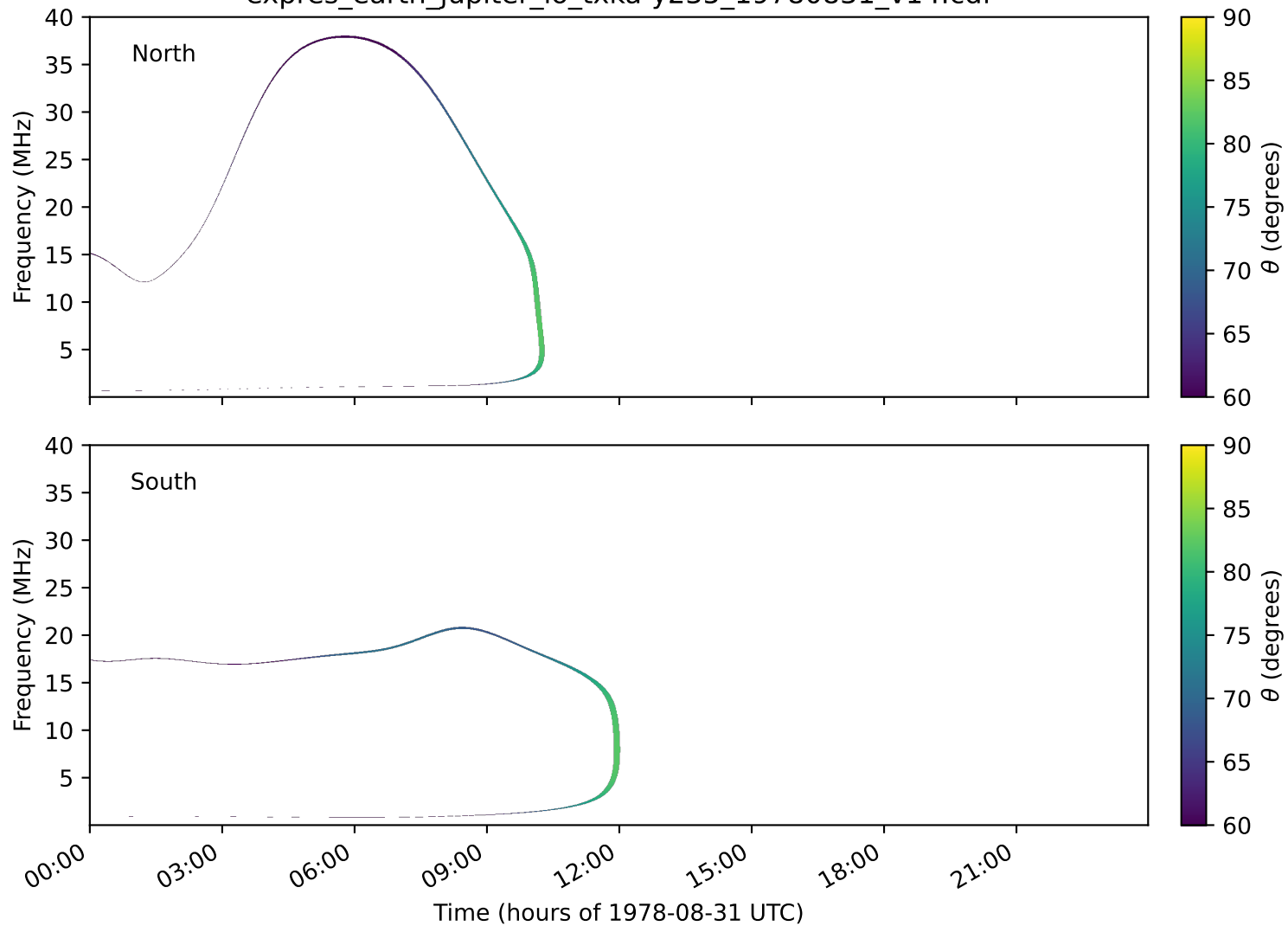
expres_earth_jupiter_io_txka-y235_19780831_v14.cdf
