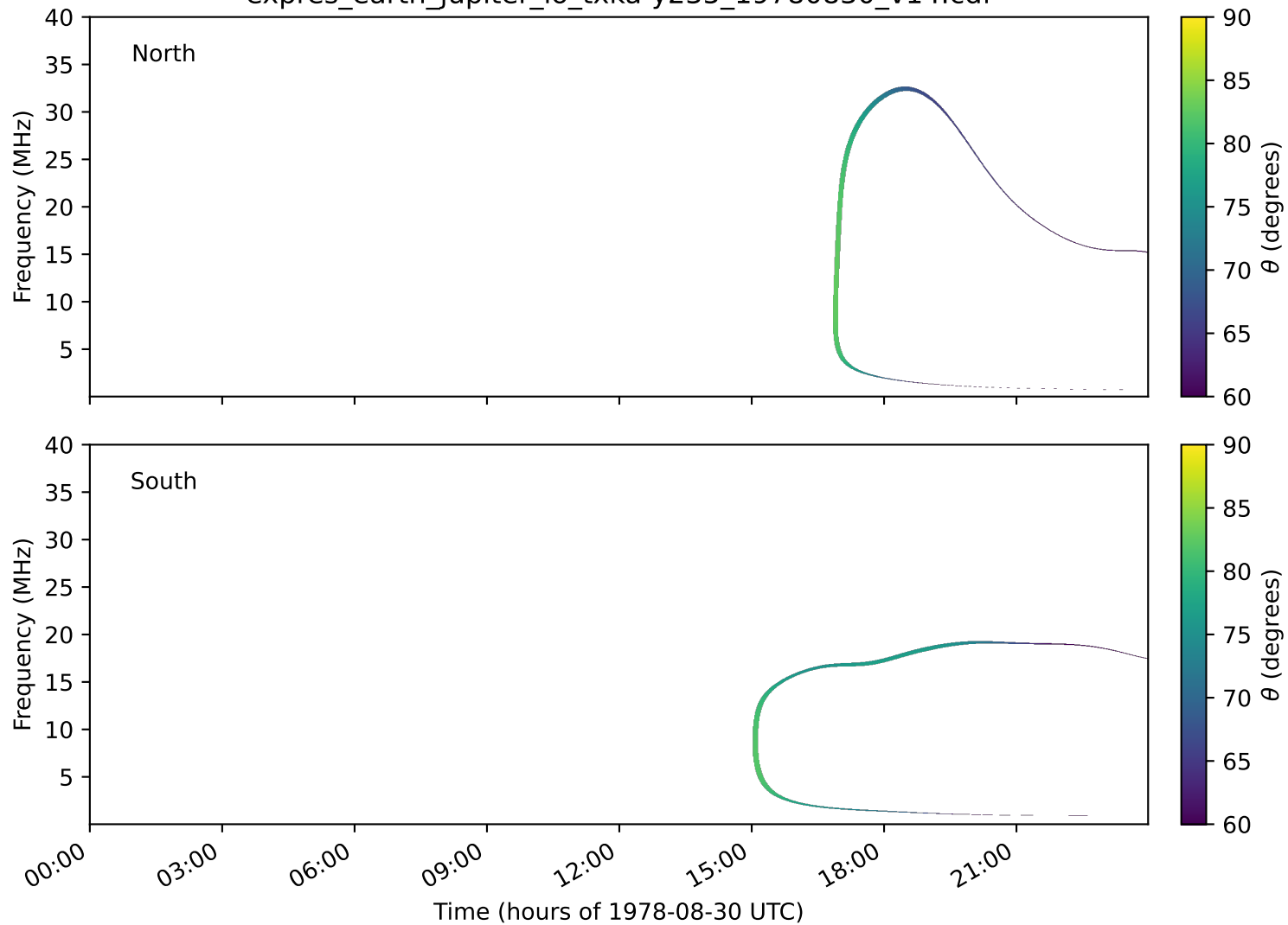
expres_earth_jupiter_io_txka-y235_19780830_v14.cdf
