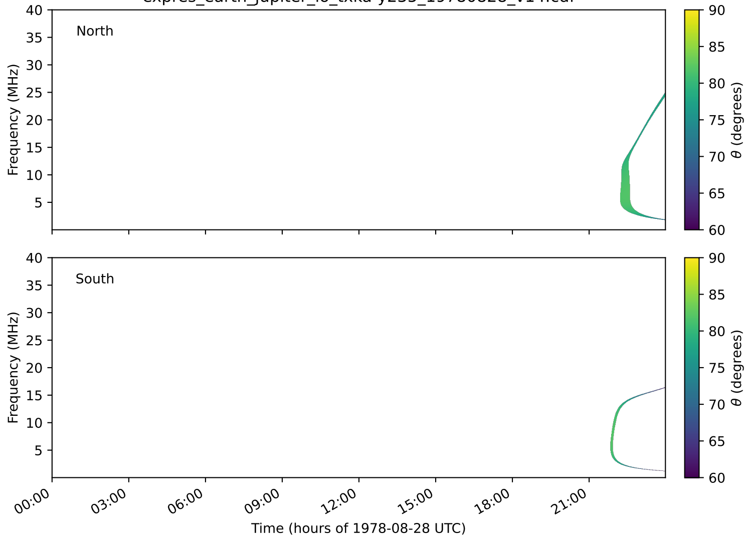
expres_earth_jupiter_io_txka-y235_19780828_v14.cdf
