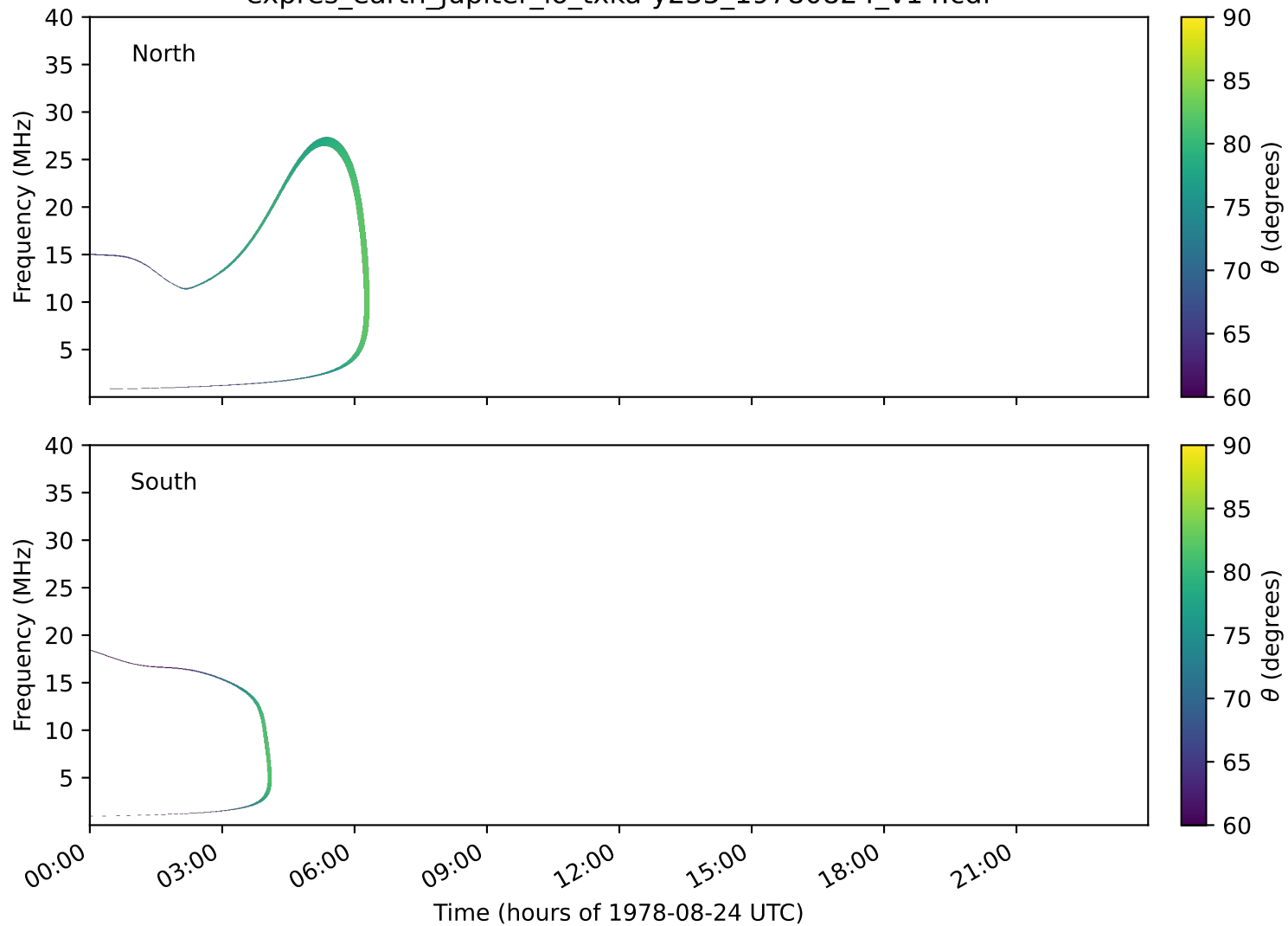
expres_earth_jupiter_io_txka-y235_19780824_v14.cdf
