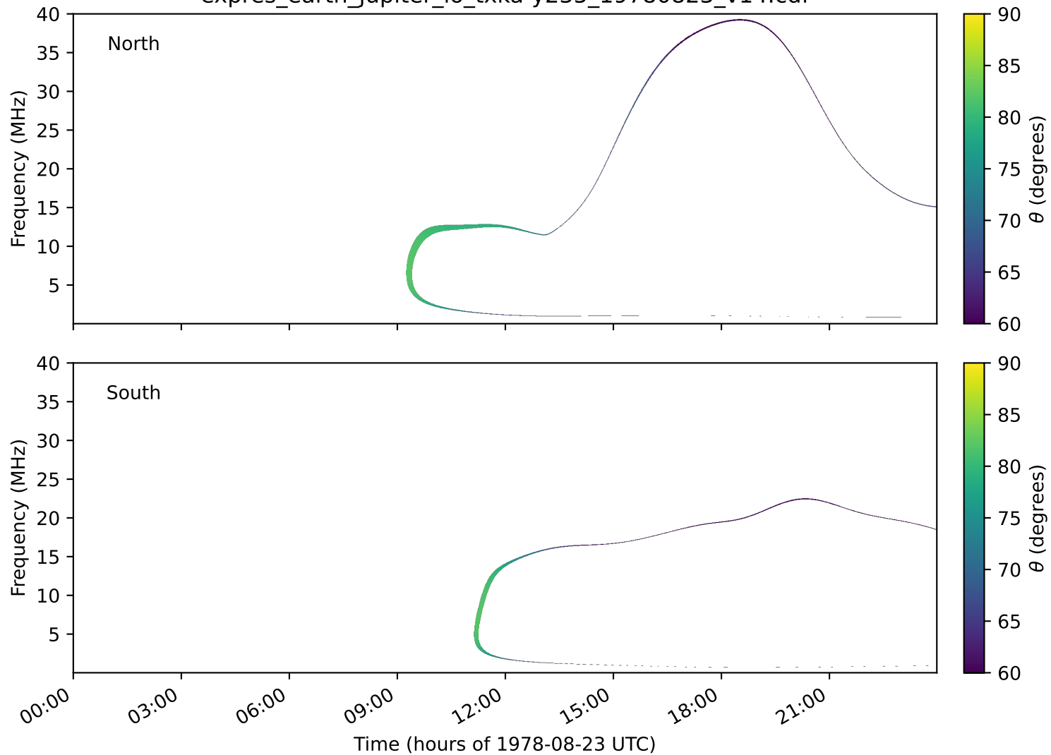
expres_earth_jupiter_io_txka-y235_19780823_v14.cdf
