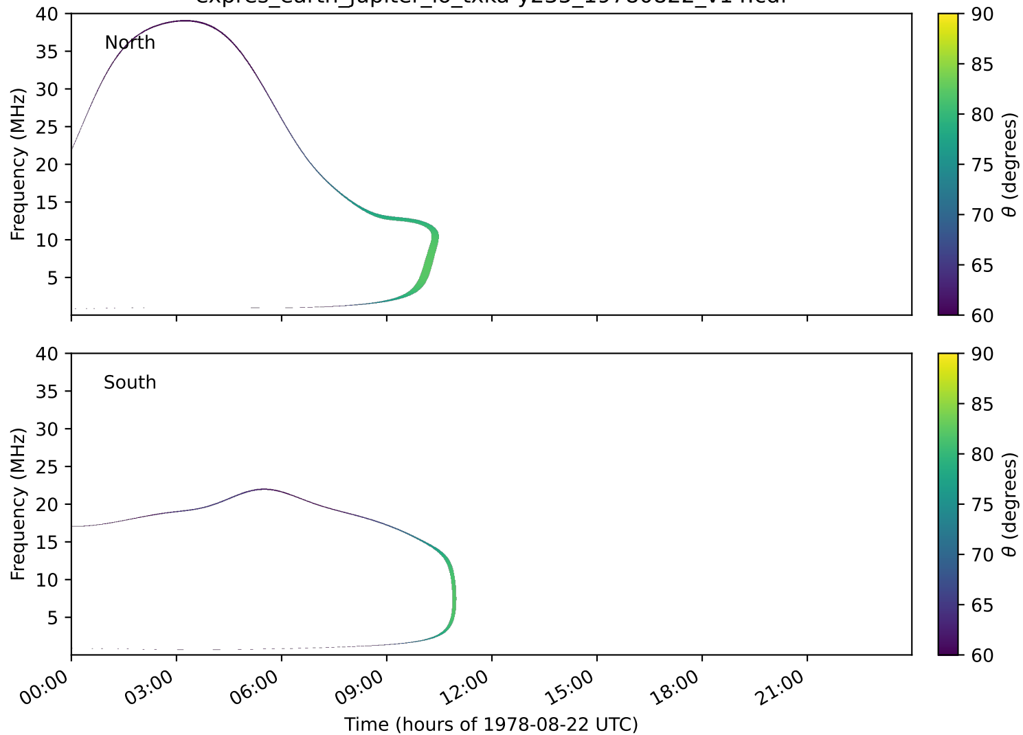
expres_earth_jupiter_io_txka-y235_19780822_v14.cdf
