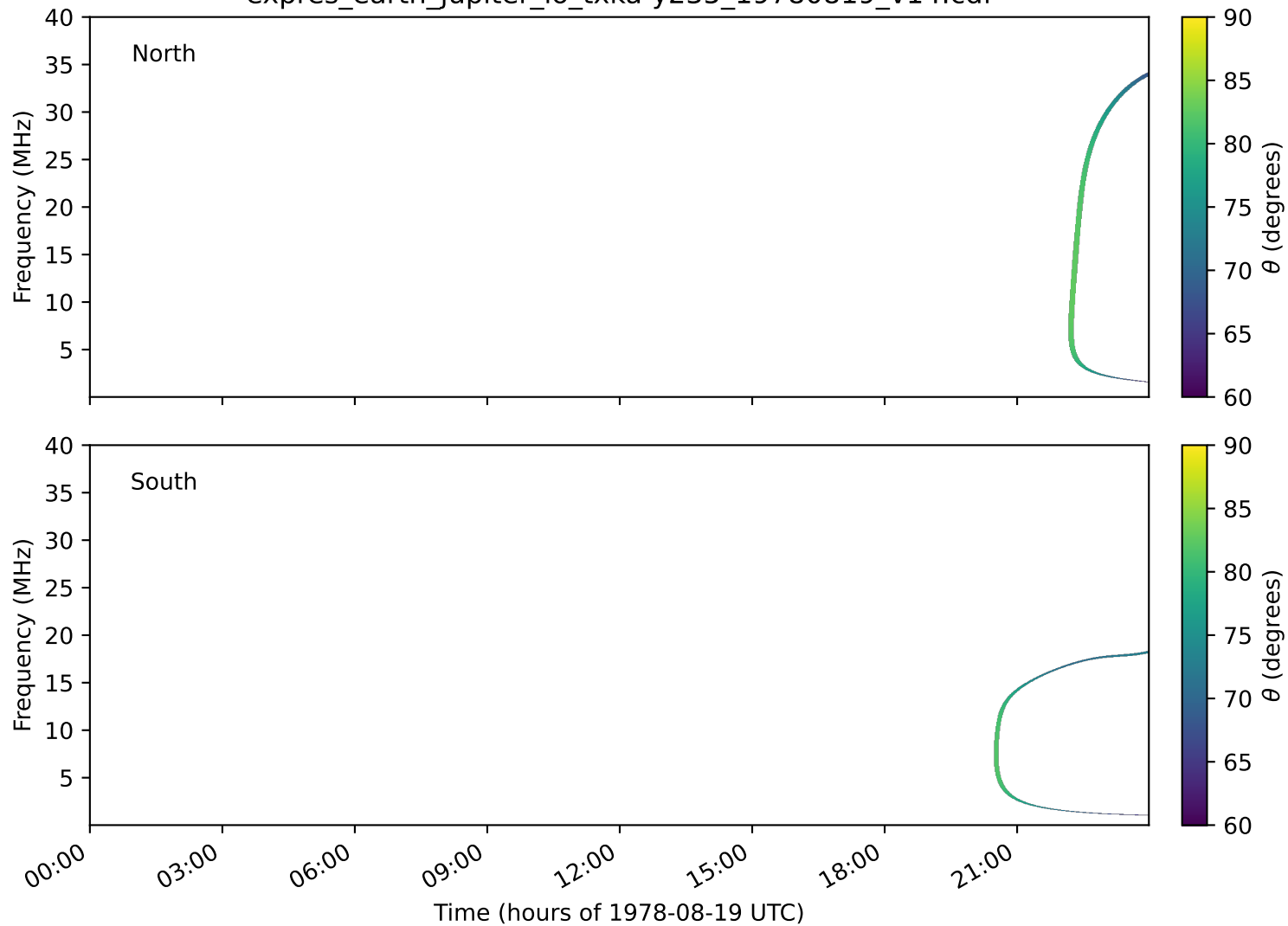
expres_earth_jupiter_io_txka-y235_19780819_v14.cdf
