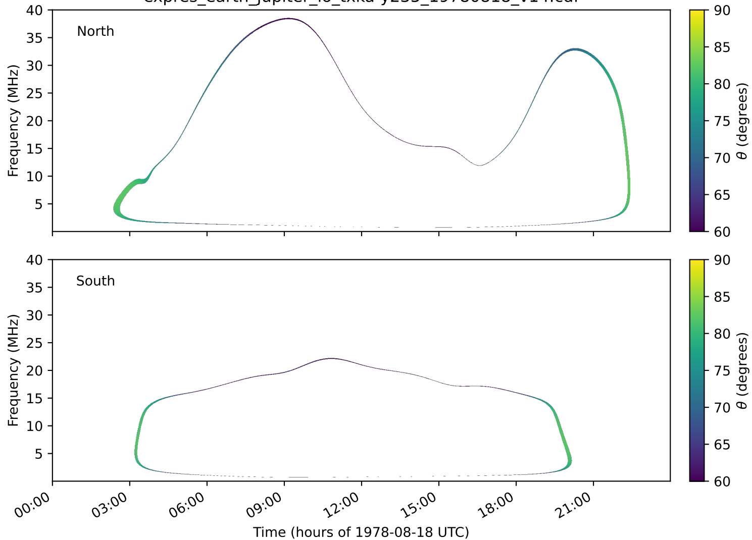
expres_earth_jupiter_io_txka-y235_19780818_v14.cdf
