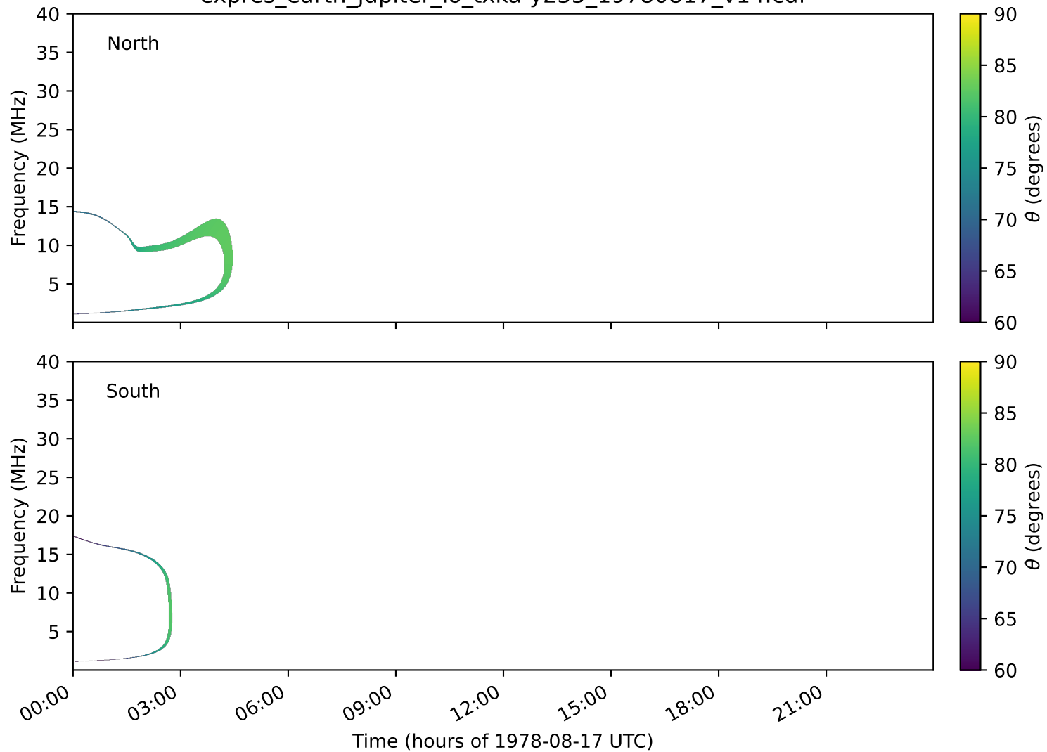
expres_earth_jupiter_io_txka-y235_19780817_v14.cdf
