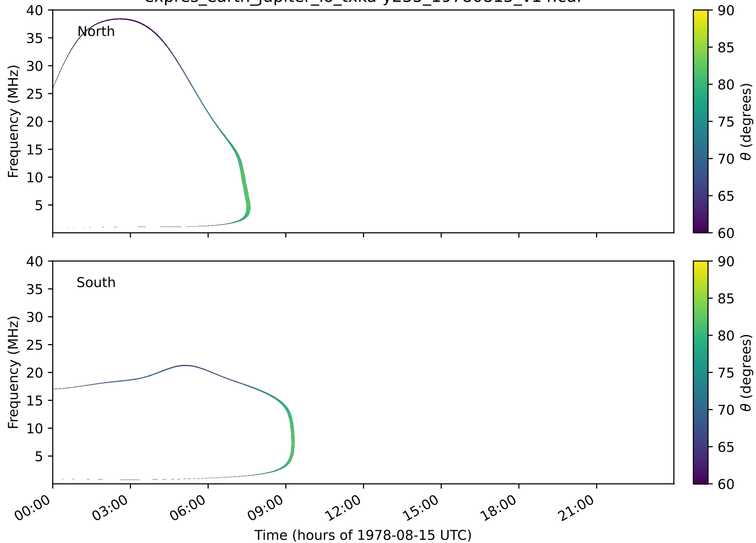
expres_earth_jupiter_io_txka-y235_19780815_v14.cdf
