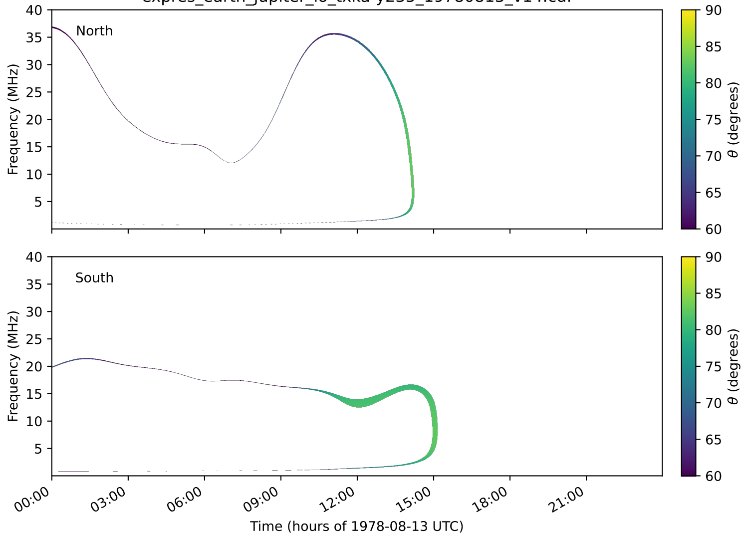
expres_earth_jupiter_io_txka-y235_19780813_v14.cdf
