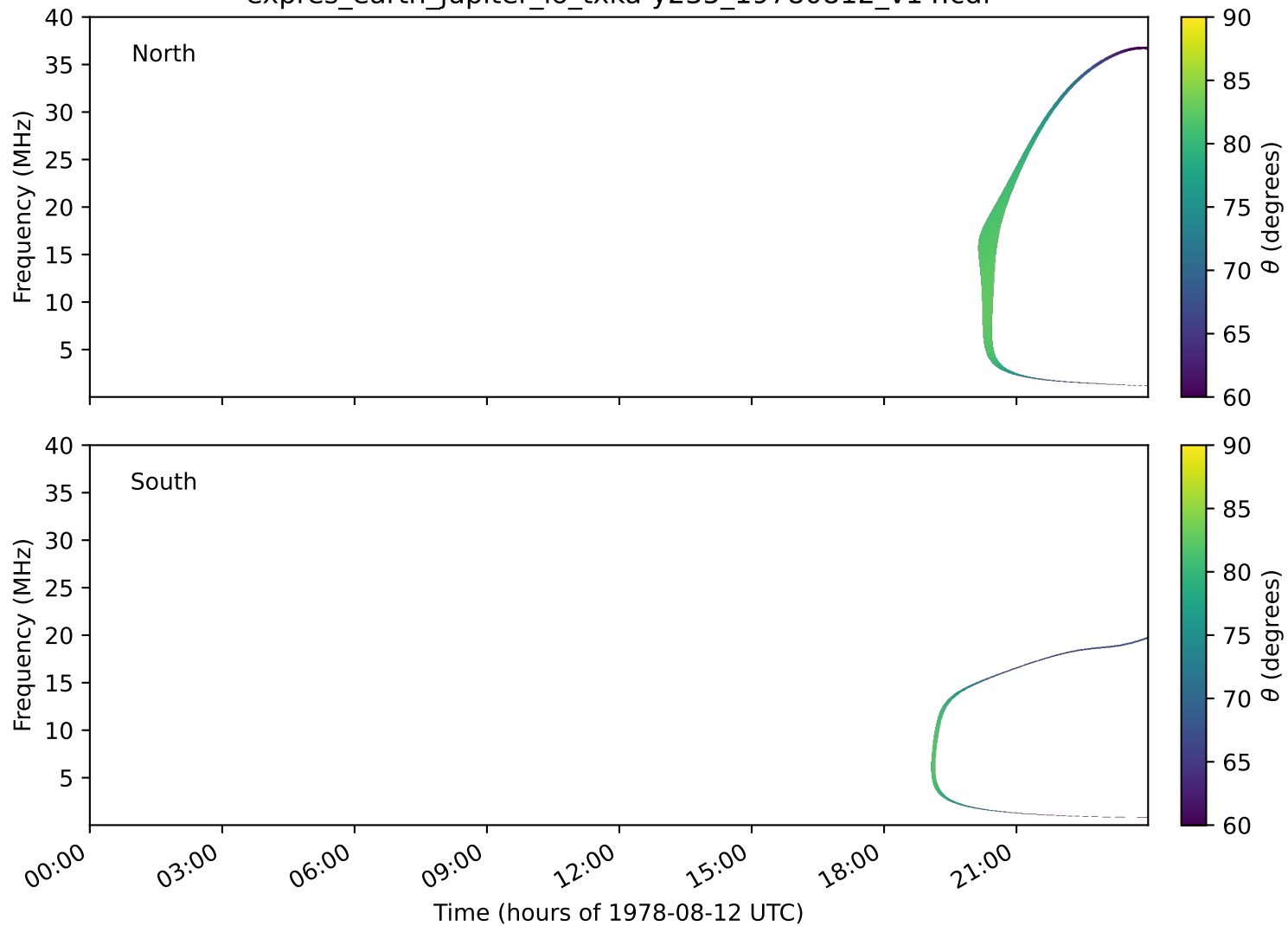
expres_earth_jupiter_io_txka-y235_19780812_v14.cdf
