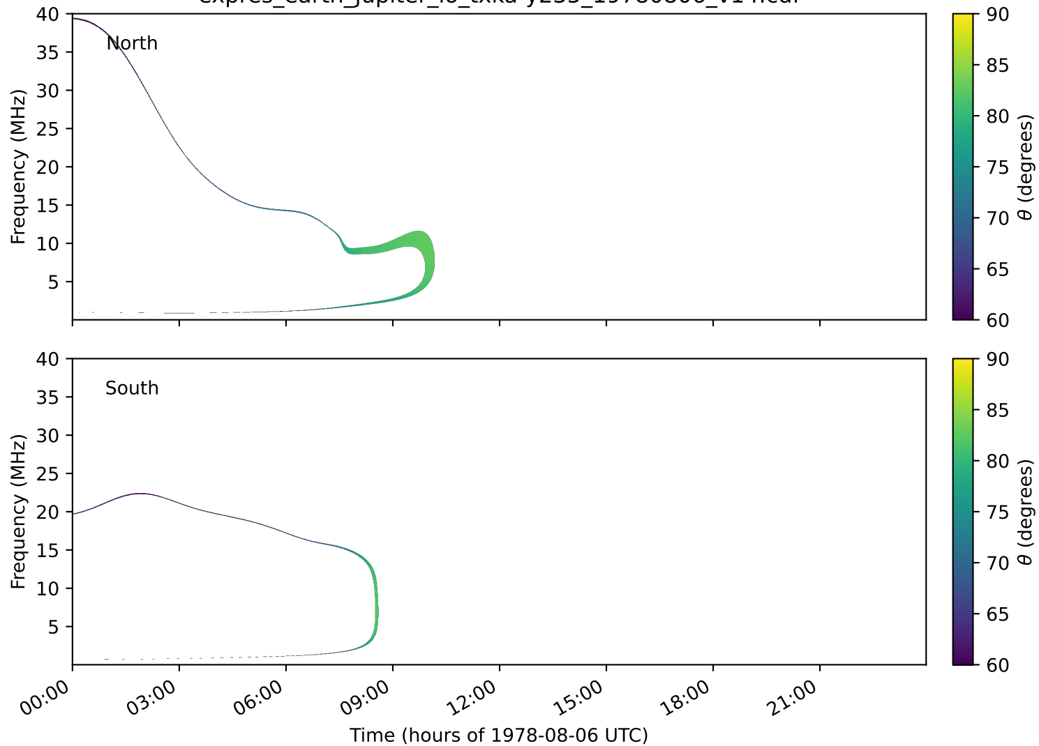
expres_earth_jupiter_io_txka-y235_19780806_v14.cdf
