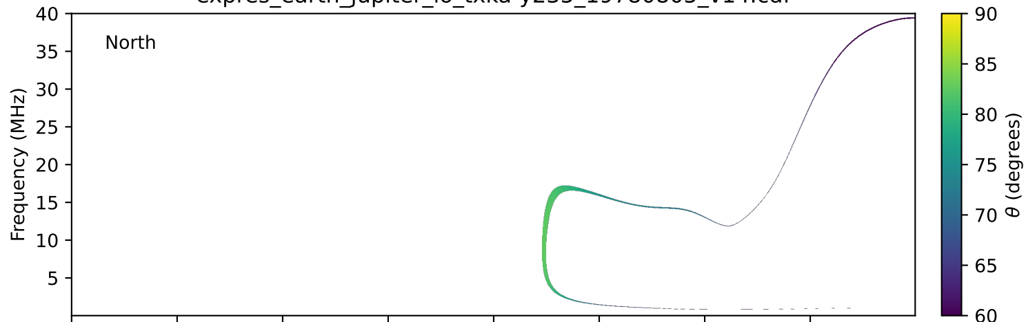
expres_earth_jupiter_io_txka-y235_19780805_v14.cdf
