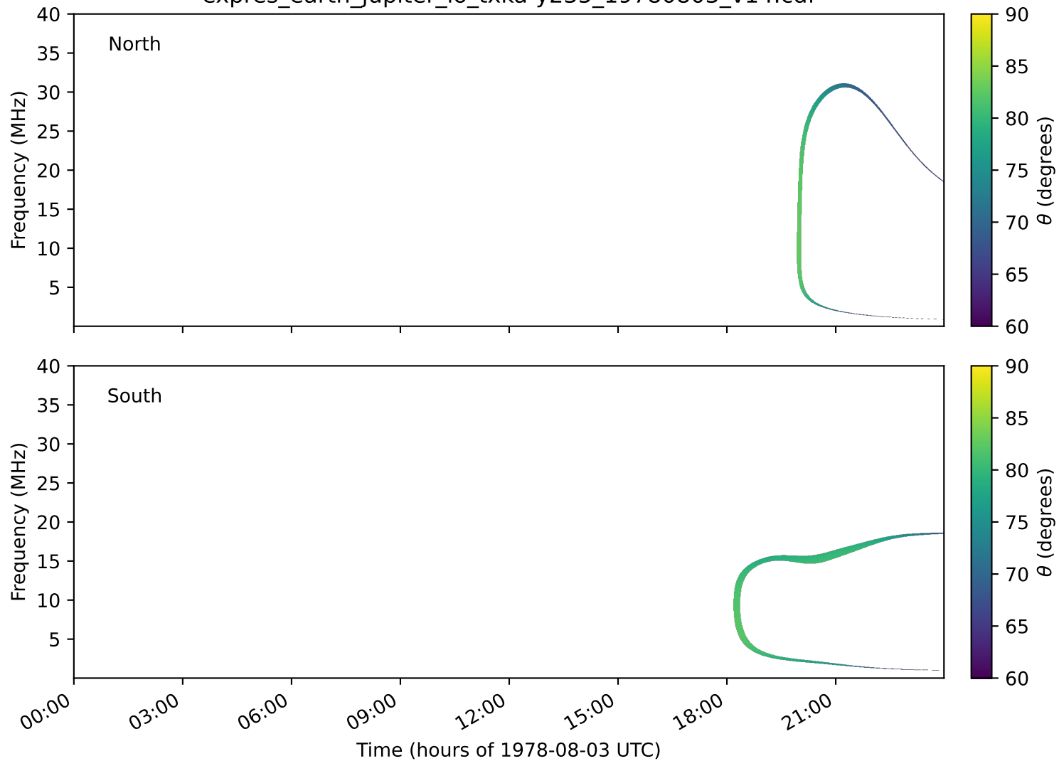
expres_earth_jupiter_io_txka-y235_19780803_v14.cdf
