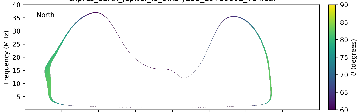
expres_earth_jupiter_io_txka-y235_19780802_v14.cdf
