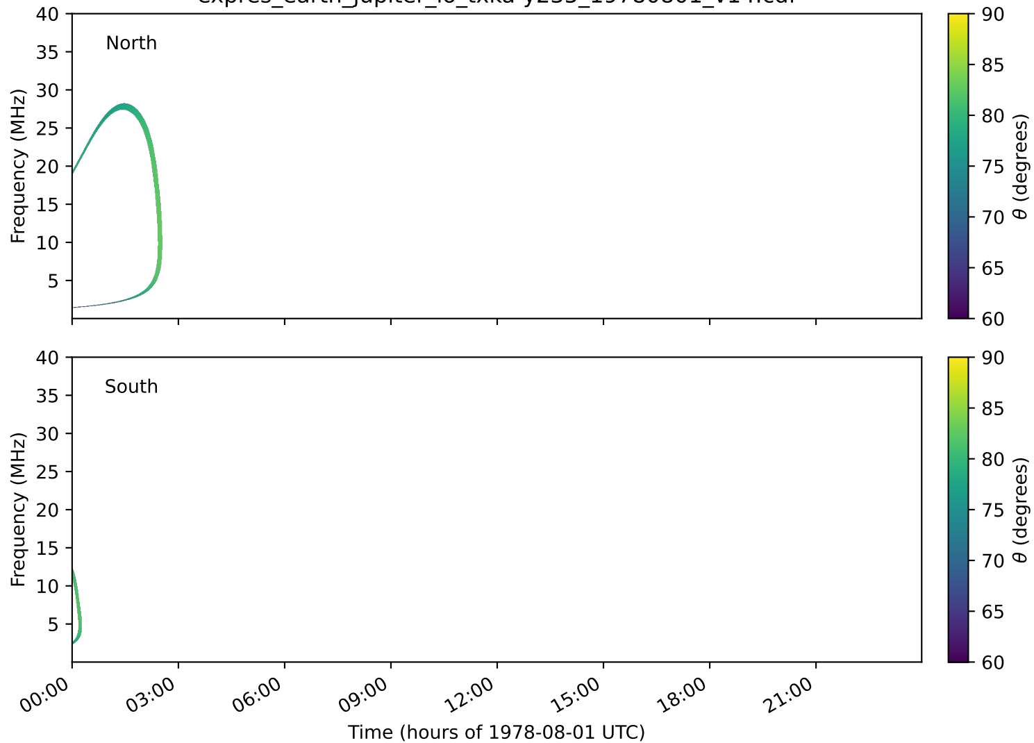
expres_earth_jupiter_io_txka-y235_19780801_v14.cdf
