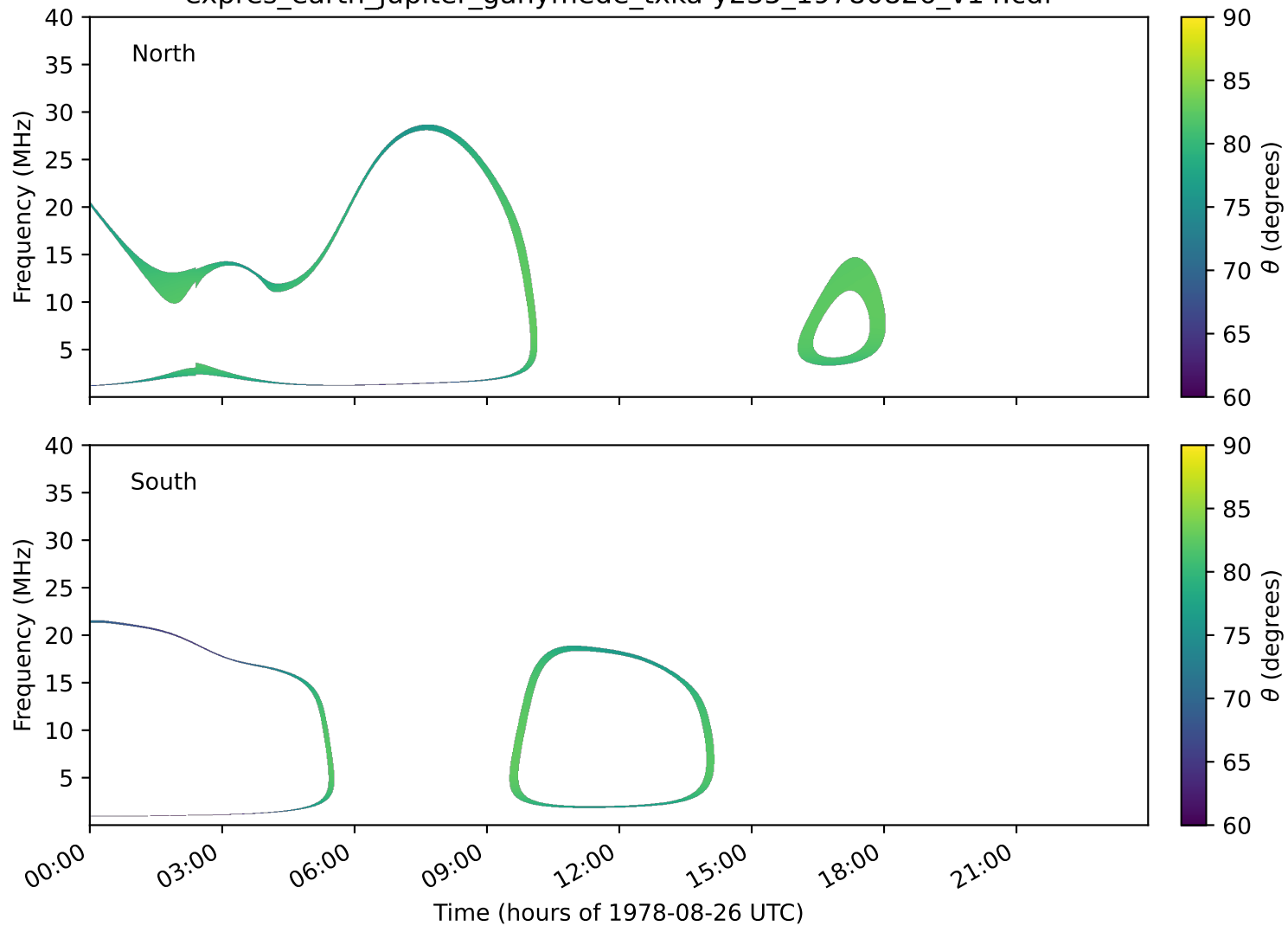
expres_earth_jupiter_ganymede_txka-y235_19780826_v14.cdf
