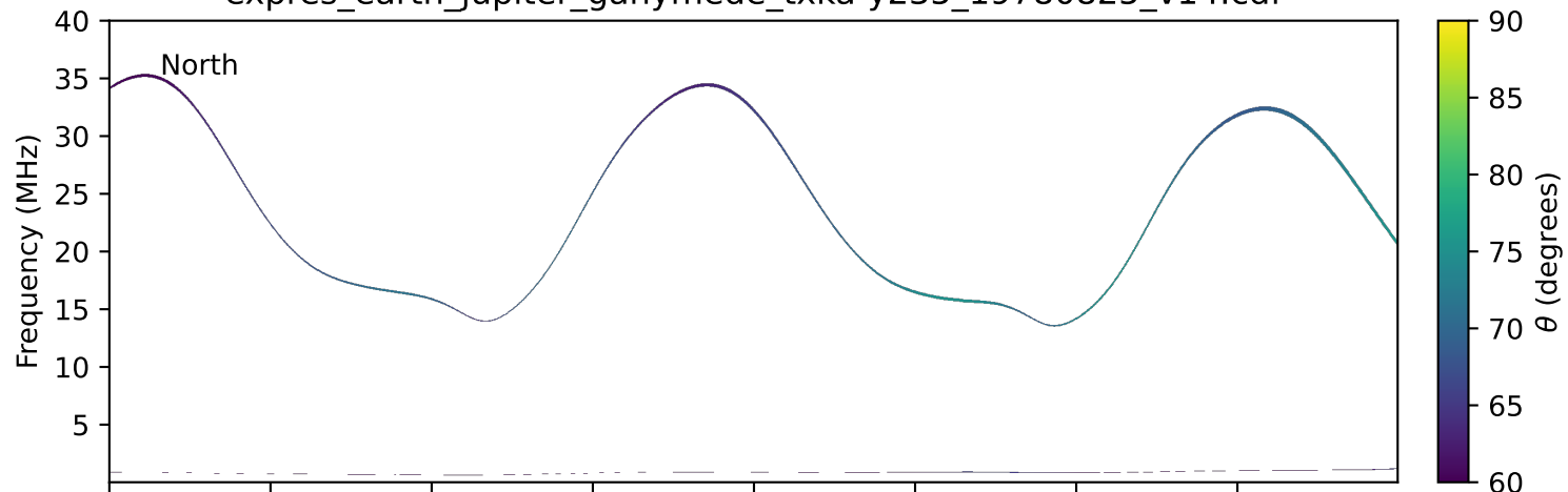
expres_earth_jupiter_ganymede_txka-y235_19780825_v14.cdf
