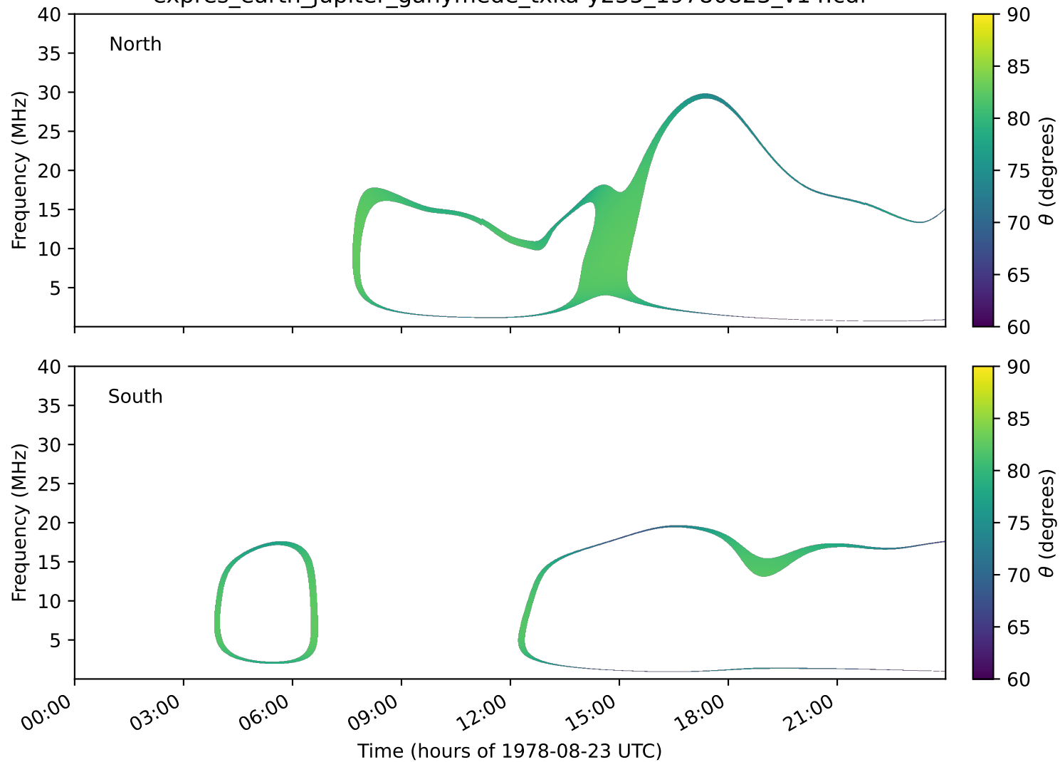
expres_earth_jupiter_ganymede_txka-y235_19780823_v14.cdf
