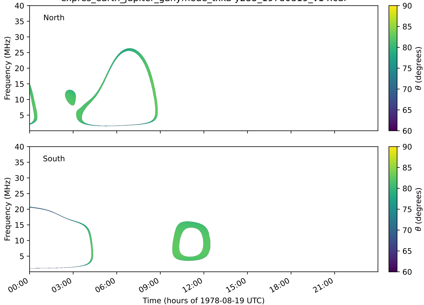
expres_earth_jupiter_ganymede_txka-y235_19780819_v14.cdf
