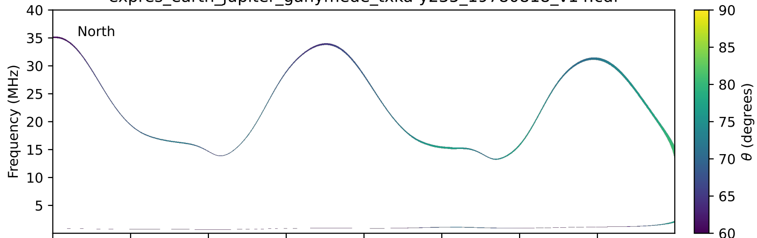
expres_earth_jupiter_ganymede_txka-y235_19780818_v14.cdf
