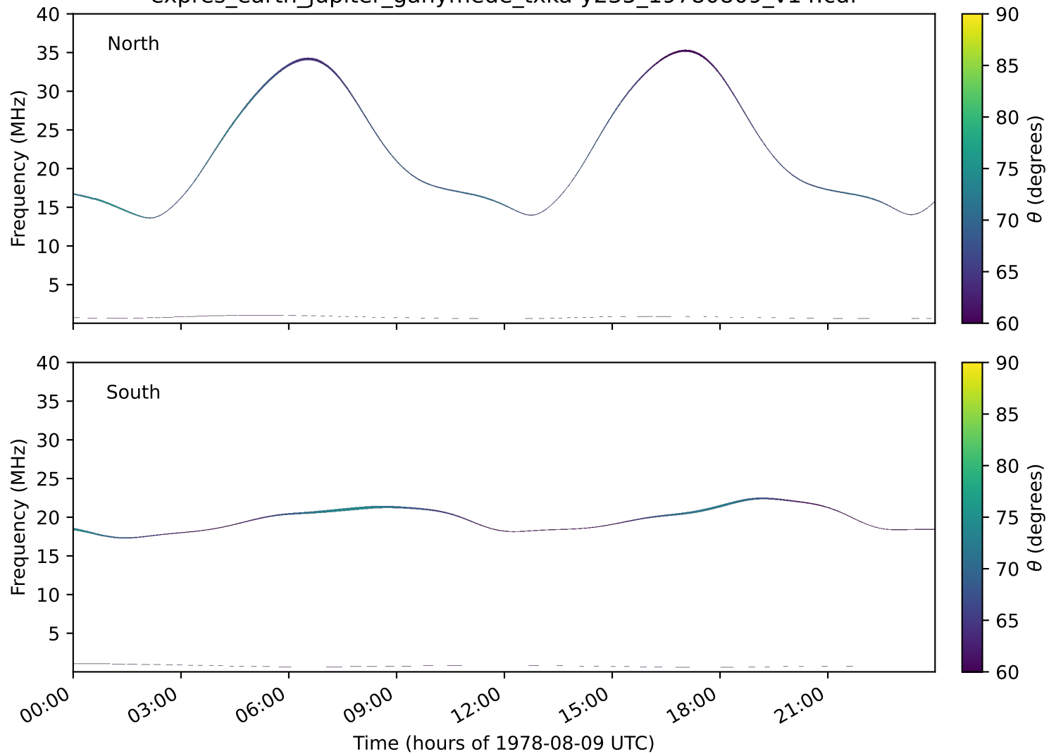
expres_earth_jupiter_ganymede_txka-y235_19780809_v14.cdf
