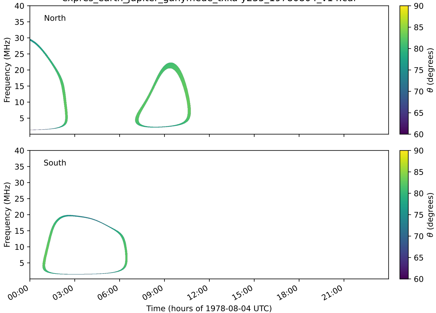
expres_earth_jupiter_ganymede_txka-y235_19780804_v14.cdf
