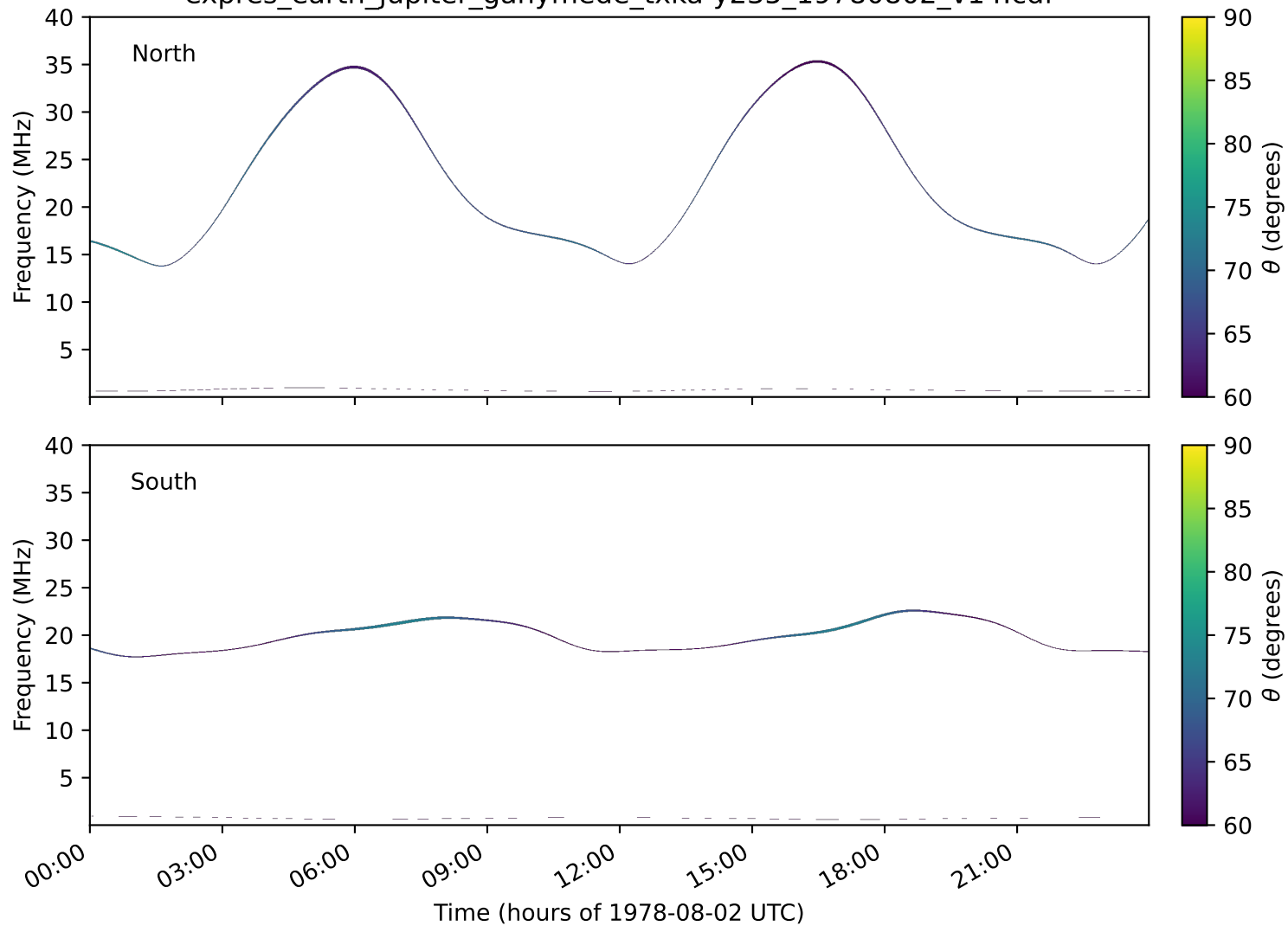
expres_earth_jupiter_ganymede_txka-y235_19780802_v14.cdf
